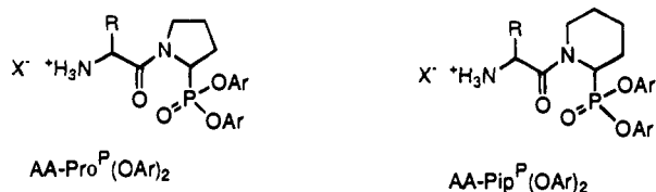
Figure 1. Structures of Pro- or Pip-containing dipeptide phosphonates, where R is the side chain of Ala, Phe, or Lys and Ar is phenyl, 4-chlorophenyl, or 4-fluorophenyl.
