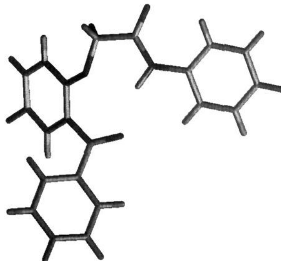
Figure 1. Crystal structure of 1h .
