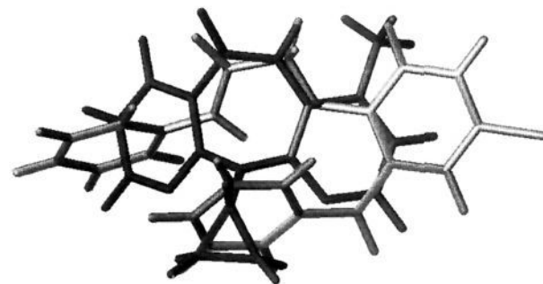
Figure 3. Proposed overlay of 1g with nevirapine.
