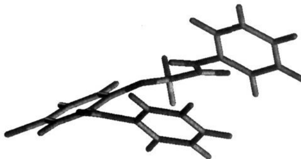
Figure 2. Proposed binding conformation of 1g .
