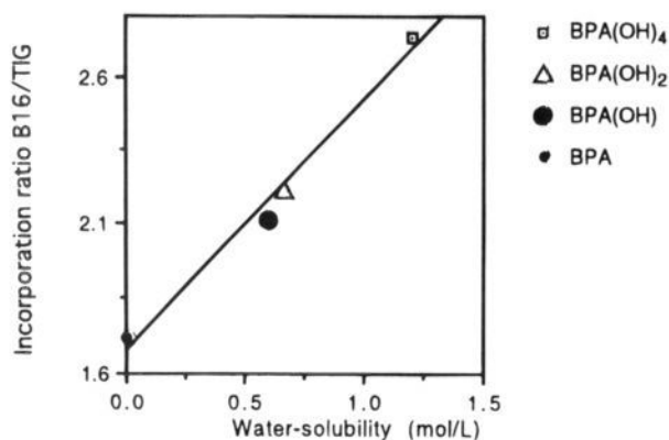
Figure 3. Relationship between water solubility and boron uptake.
