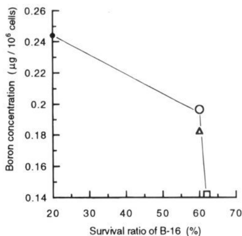
Figure 4. Relationship between cellular uptake at 24 h and cell survival ratio of B-16: (○) BPA, (○) BPA(OH), (△) BPA(OH) 2 , and (□) BPA(OH) 4 .
