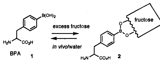
Scheme 1. BPA and Its Fructose Complex
