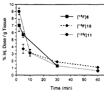
Figure 2. Time course in mice of [ 18 F]6, [ 18 F]10, and [ 125 I]11 radioactivity for whole brain. Data are expressed as % injected dose/g of tissue at the specified times points post injection and are the average of four animals. Error bars denote standard deviation.
