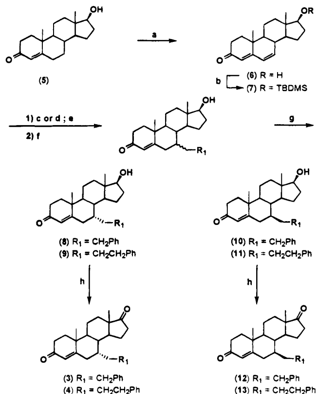
Figure 1. Structures of 7 \alpha -APTA and the 7 \alpha -arylaliphatic-substituted androstenediones.
