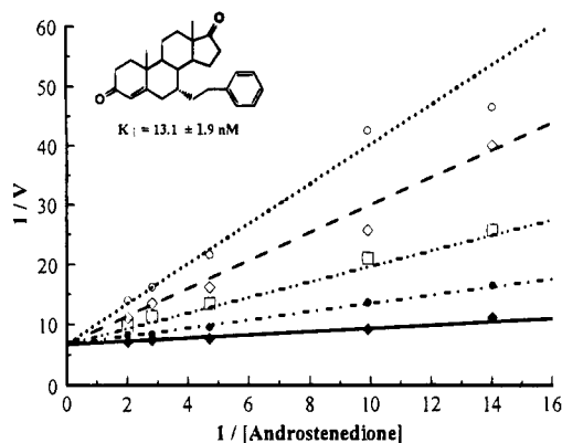
Figure 5. Lineweaver–Burk plot of aromatase inhibition by compound 3 . Various concentrations of androstenedione (70–500 nM) were incubated with microsomal enzyme preparations at inhibitor concentrations of 0 nM ( \blacklozenge ), 20 nM ( \bullet ), 50 nM ( \square ), 100 nM ( \diamond ), or 150 nM ( \circ ). Velocity is expressed as nmol product per \mu\text{g} protein per minute and 1/[\text{androstenedione}] values have units of \mu\text{mol}^{-1} . Each point represents the average of three determinations with less than 10% variation from the mean.
