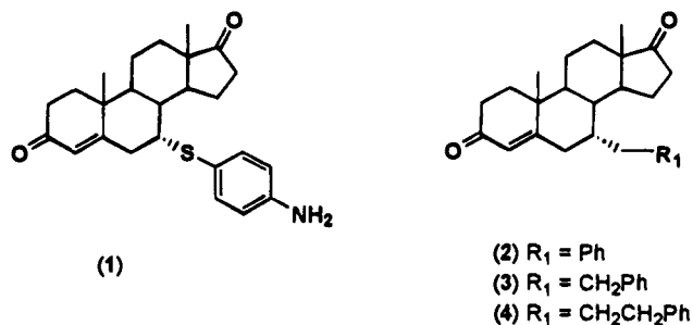
Figure 1. Structures of 7 \alpha -APTA and the 7 \alpha -arylaliphatic-substituted androstenediones.
