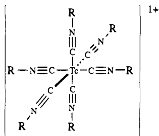
Figure 1. General structure of hexakis(R-isonitrile)technetium(I) complexes.
