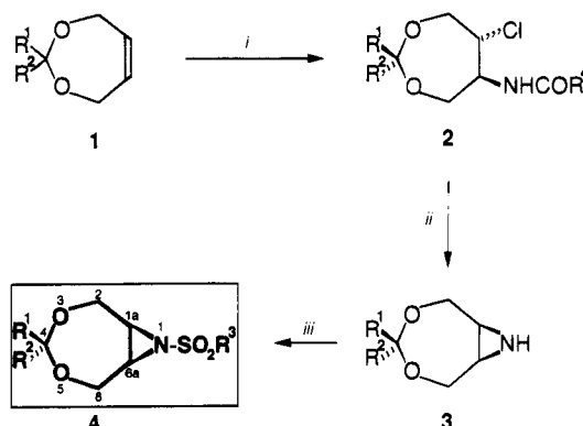
Scheme 1 a
