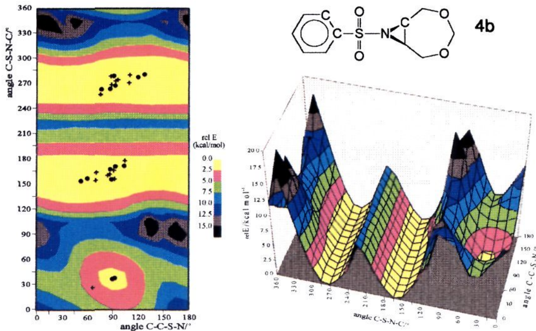
Figure 5. Relative strain energy ( E_{rel} = E - E_{min} ) contour plot of the model compound 4b obtained by varying together torsional angles C-C-S-N and C-S-N-C by 15° steps and the corresponding 3D representation. Dots: the studied 4 from X-ray. Pluses: other sulfonylaziridines filed in ref 15.
