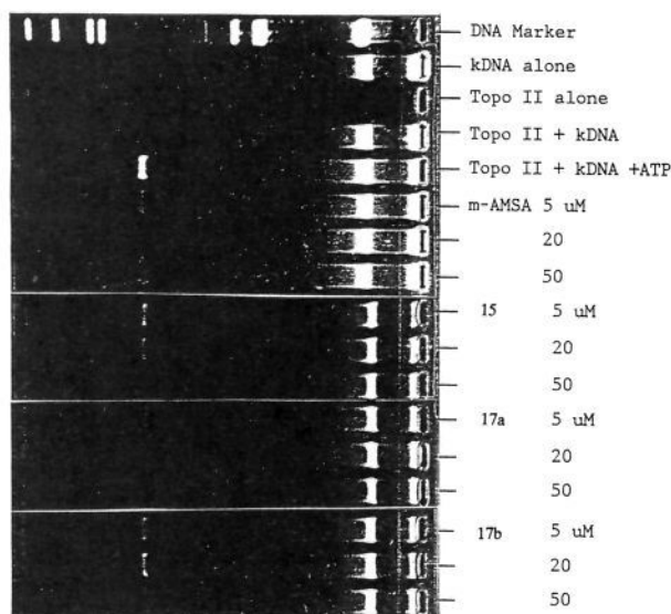
Figure 2. Inhibition of Topo II-mediated k-DNA decatenation by AHMA ( 15 ), 17a,b , and m -AMSA using purified Topo II from calf thymus. 20 Electrophoresis was carried out on 1% agarose in TBE buffer as described previously. 28,29
