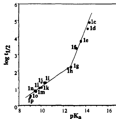
Figure 3. Brønsted relationship for the liberation of chlorzoxazone from alkyl and aryl N -(5-chloro-2-hydroxyphenyl)carbamate prodrugs 1 (experimental conditions: pH 7.40 phosphate buffer, 37 °C). Linear regression equations relevant to these data are \log t_{1/2} = 0.46pK_a(\text{ROH}) - 3.55 ( r = 0.991 , s = 0.02 ) for aryl and trihalogenoethyl esters and \log t_{1/2} = 1.46pK_a(\text{ROH}) - 16.03 ( r = 0.988 , s = 0.12 ) for alkyl esters. Half-lives values for prodrugs 1a ( t_{1/2} = 73 days) and 1b ( t_{1/2} = 290 days) have been extrapolated from the latter equation using the pK a values of methanol and ethanol, respectively.
