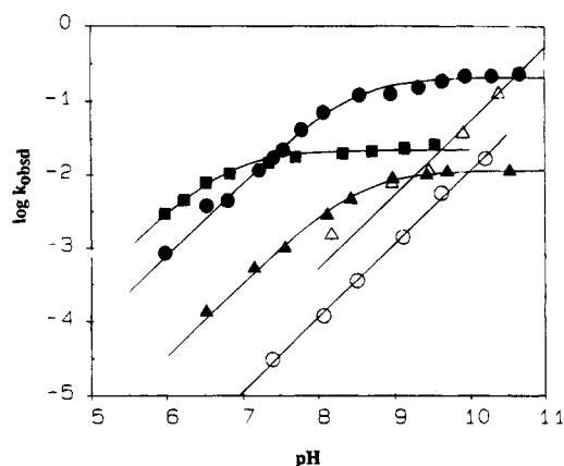
Figure 1. Plots of \log k_{\text{obsd}} vs pH for the hydrolysis of prodrug 1g (▲), mutual prodrugs 1m (●), 2 (■), and 5 (○), and O -methyl derivative 14 (△). All kinetics were carried out at 25 °C and ionic strength \mu = 0.5 M with KCl except for 5 ( T = 37 °C, \mu = 1.0 M).
