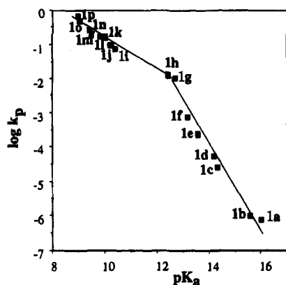
Figure 2. Brønsted relationship for the cyclization reaction of alkyl and aryl N -(5-chloro-2-hydroxyphenyl)carbamates 1 to chlorzoxazone (experimental conditions: pH 10–11 carbonate buffer, 25 °C).
