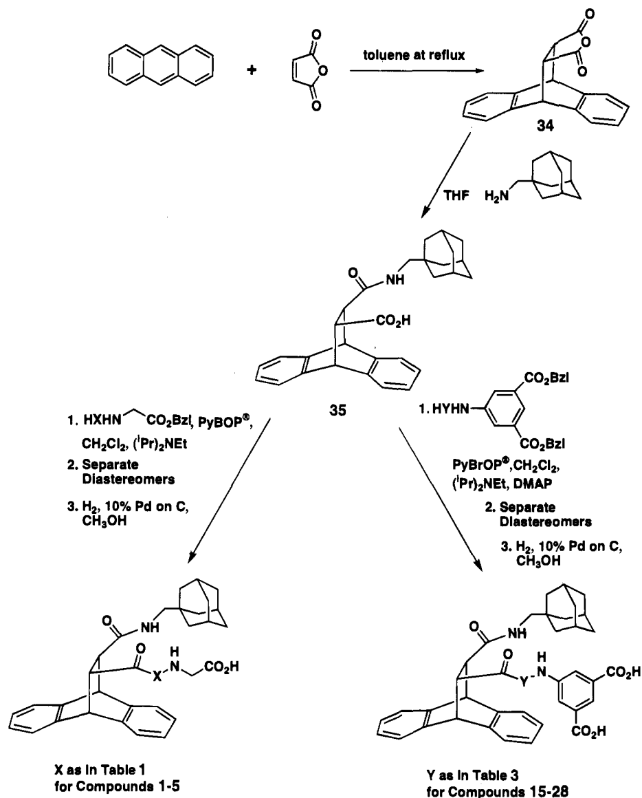
Scheme 1. Synthesis of Compounds 1–5 and 15–28
