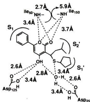
Figure 4. Interatomic distances of compound 19 binding to HIV PR as derived from the X-ray crystal structure. Distances are measured between heavy atoms.
