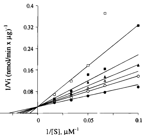
Figure 2. Double-reciprocal plot for inhibition of HIV-1 protease by compound 19 . Inhibitor concentration, nM: (□) 90, (■) 45, (△) 30, (▲) 20, (○) 13, (●) 0.0. The data are shown to fit to a competitive inhibition model by a nonlinear least-squares algorithm, with K m = 34 ± 4.3 μM (standard error), k cat = 15 ± 1.0 s -1 , and K i = 33 ± 3.9 nM.
