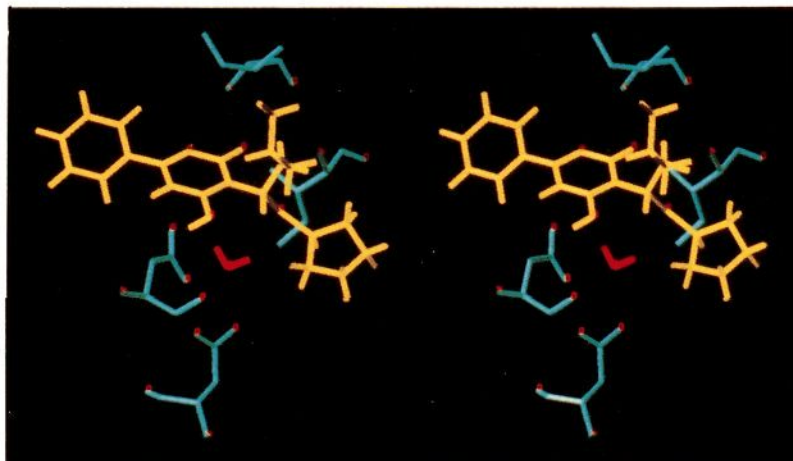
Figure 3. Relaxed stereorepresentation of the X-ray crystal structure (yellow) of compound 19 bound to HIV PR. Asp25/125 and Ile50/150 from the crystal complex are shown in cyan, and bridged water is shown in red.
