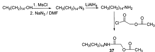
Scheme 2. Synthesis of N -(2-Acetoxyacetyl)pentadecylamine 37
