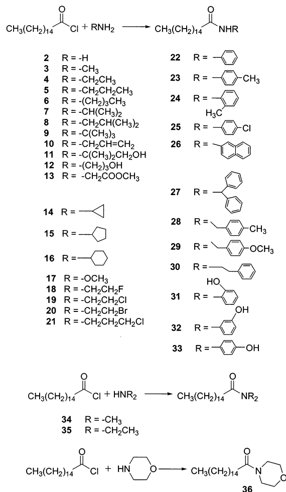
Scheme 2. Synthesis of N -(2-Acetoxyacetyl)pentadecylamine 37
