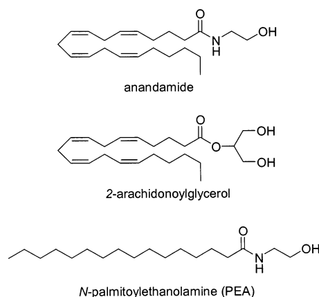
Figure 1. Structures of endocannabinoids and related endogenous lipids.
