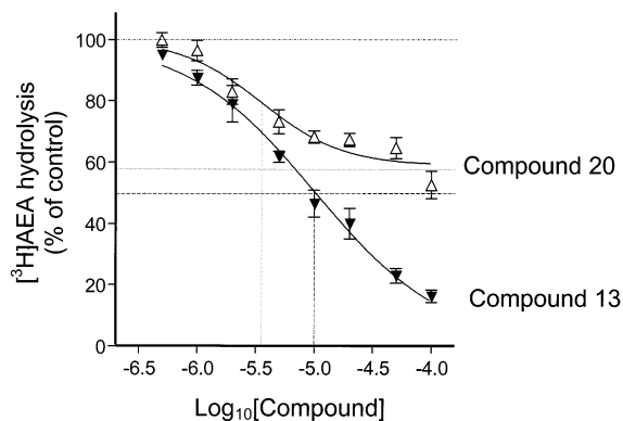
Figure 2. Inhibition of 2 \mu\text{M} [ ^3\text{H} ]-AEA metabolism by compounds 13 (filled triangles) and 20 (open triangles). For compound 13 , analysis of the data indicated that the maximum inhibition was not significantly different from 100% (i.e., 95% confidence limits of the minimum activity remaining straddled 0%). The pI_{50} value of the inhibitable fraction is thus the concentration of the compound that produces 50% inhibition of [ ^3\text{H} ]-AEA metabolism (shown as broken line in the figure). For compound 20 , the analysis indicated that the curve reached a plateau at a value significantly higher than zero (59%, 95% confidence limits 52–66%). Thus, the inhibitable fraction of the activity is 41%. The pI_{50} value of the inhibitable fraction is thus the concentration of the compound that produces 20.5% inhibition of [ ^3\text{H} ]-AEA metabolism (shown as \cdots in the figure). The data are the mean \pm SEM, n = 3 .
