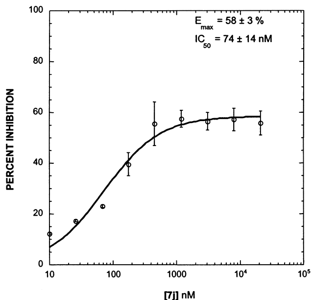
Figure 1. Concentration–response curve for inhibition of SNC-80 stimulated [ ^{35}\text{S} ]GTP- \gamma -S binding by 7j .
