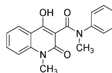
Roquinimex ( 1b )
