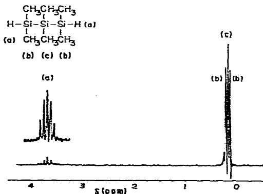
Fig. 1. NMR spectrum of 1,1,2,2,3,3-hexamethyltrisilane (VII).
