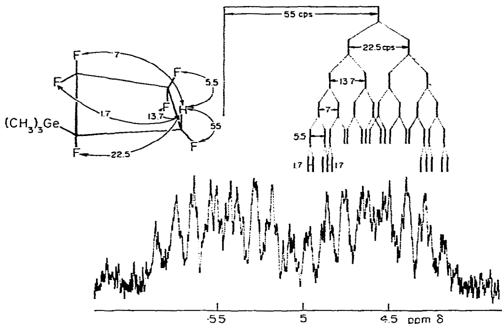
Fig. 2. ^1\text{H} NMR spectrum of (\text{CH}_3)_3\text{GeCFCFHCF}_2\text{CF}_2 .
