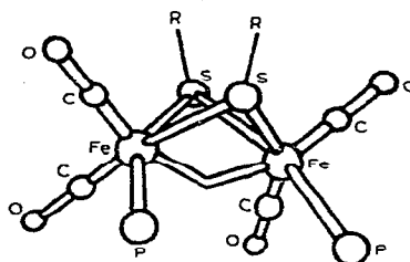
Isomer B
