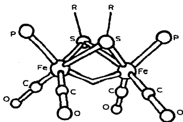
Isomer A
