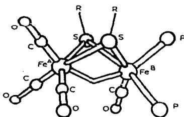
Isomer C
