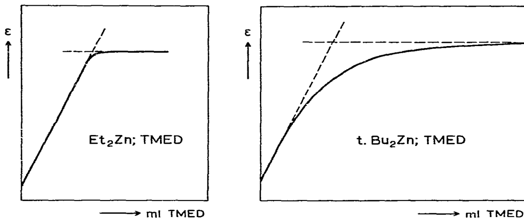
Fig. 1. Dielectric constant titration of \text{Et}_2\text{Zn} and tert-Bu 2 Zn with TMED in benzene
