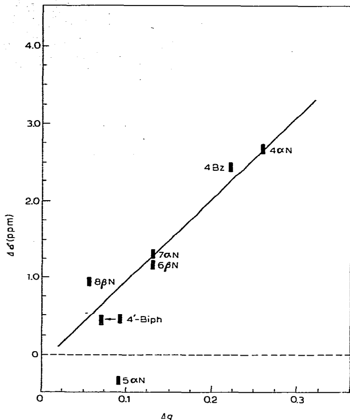
Fig. 1. Plot of \Delta q (SCFMO) versus \Delta\delta [(CH 3 ) 3 CCH 2 → (CH 3 ) 3 SnCH 2 ] for various dispositions in benzene, naphthalene and biphenyl. The 4-biphenyl value has been corrected for non-coplanarity of the rings. Correlation coefficient r = 0.98 at 99% confidence level.
