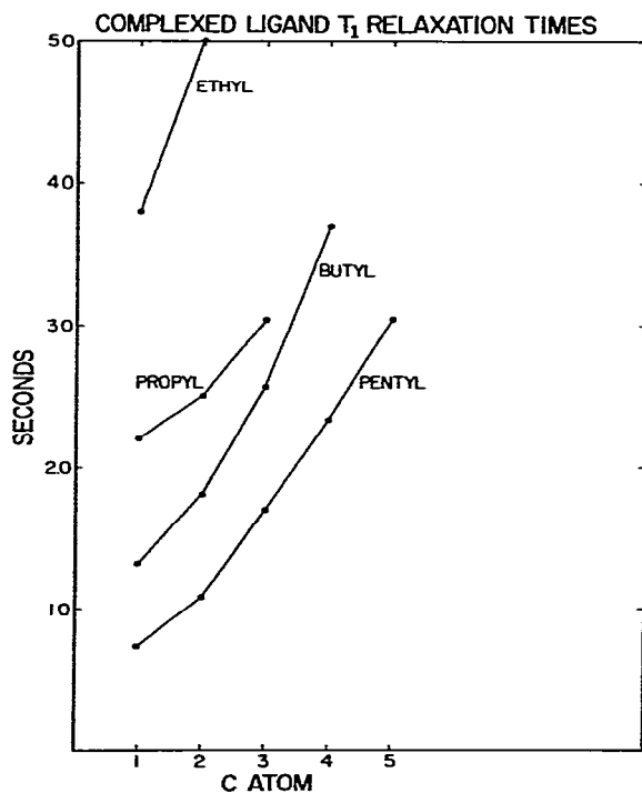
Fig. 2. A plot of the ^{13}\text{C} NMR spin-lattice ( T_1 ) relaxation time in seconds versus the position along the alkyl chain in \text{LNi}(\text{CO})_3 complexes of \text{P}(\text{CH}_2)_n\text{CH}_3 ligands, ( n = 1-4 ). C(1) is assigned to the carbon attached to the phosphorus atom.
