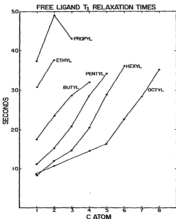
Fig. 1. A plot of the ^{13}\text{C} NMR spin-lattice ( T_1 ) relaxation time in seconds versus the position along the alkyl chain in \text{P}((\text{CH}_2)_n\text{CH}_3)_3 ligands, ( n = 1-5, 7 ). C(1) is assigned to the carbon attached to the phosphorus atom.
