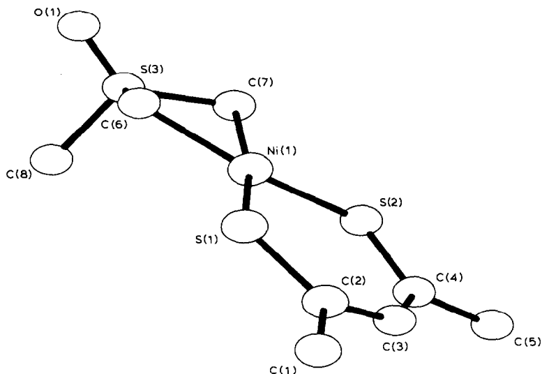
Fig. 1. PLUTO diagram of single molecule.
