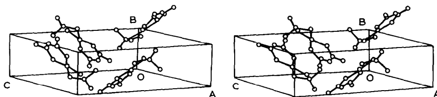
Fig. 2. PLUTO stereograph packing diagram.
