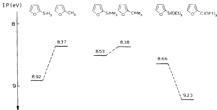
Fig. 4. Energies of \pi^* MO levels for compounds II–III, VII–VIII and IX–X.
