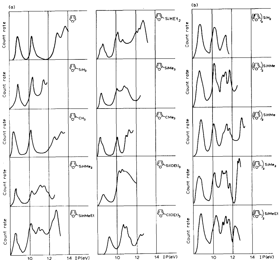
Fig. 1. a) He(I) photoelectron spectra of compounds 1–X; b) He(I) photoelectron spectra of compounds XI–XV.
