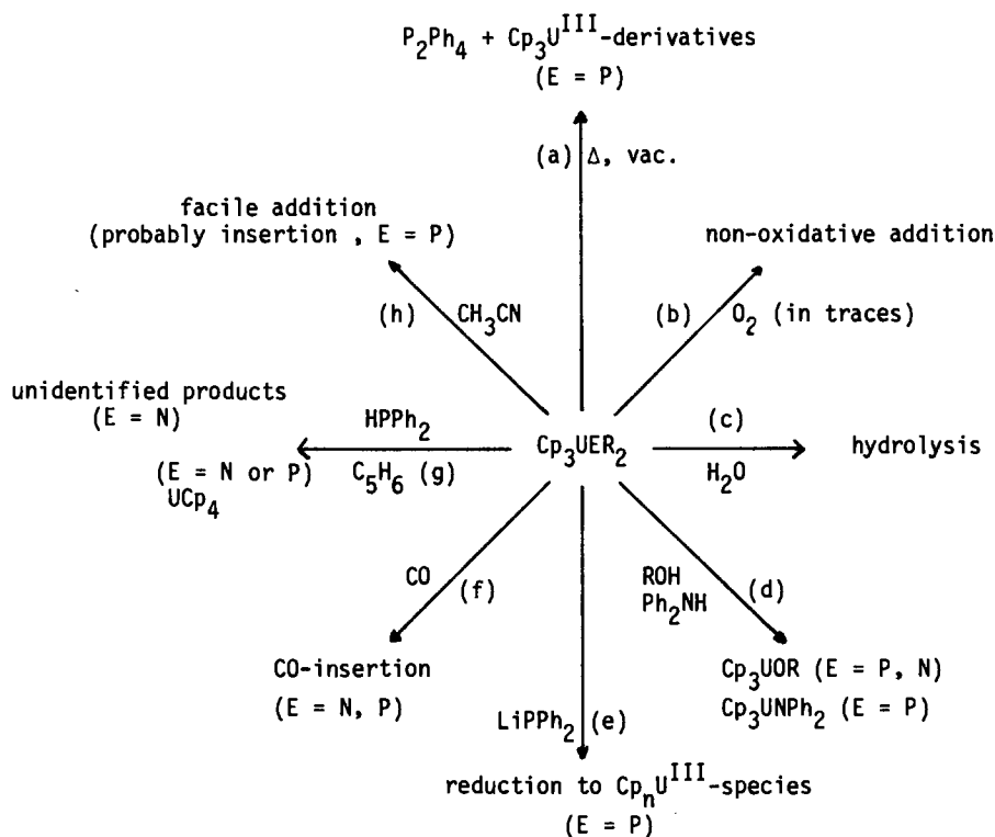
SCHEME 2. Outline of the known reactions of \text{Cp}_3\text{UER}_2 systems ( \text{E} = \text{P} or \text{N} ).
