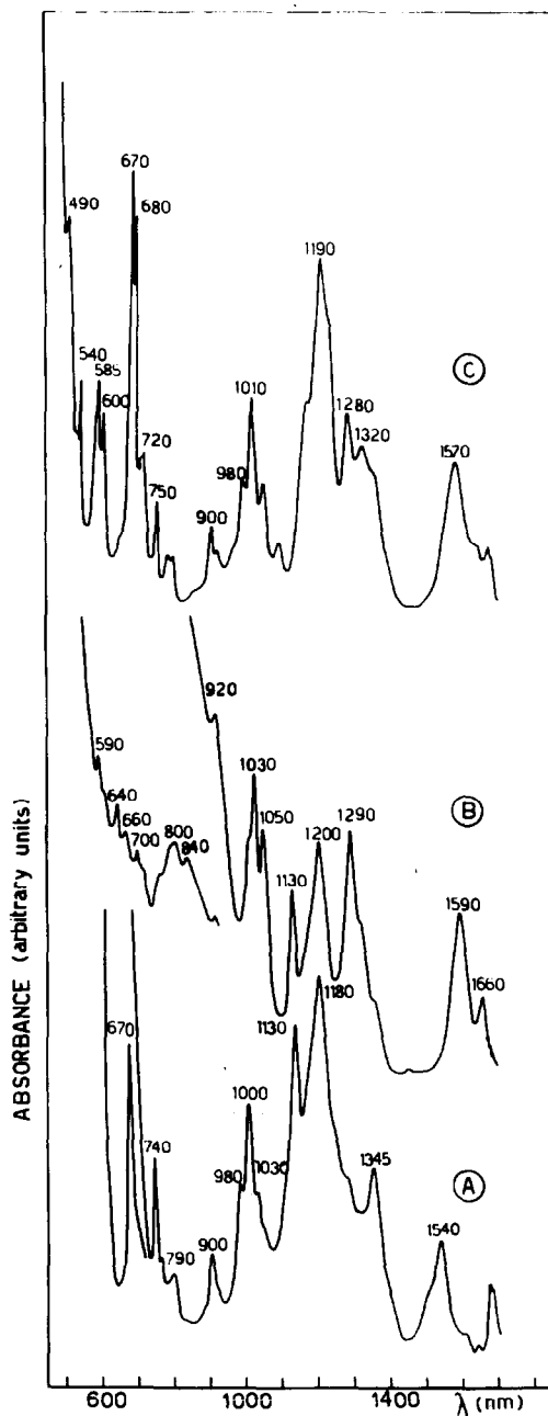
Fig. 1. Comparison of the absorption spectra of three related \text{Cp}_3\text{UX} systems (A: X = NEt 2 , B: X = PPh 2 , C: X = OPh) in the near infrared and visible (NIR-VIS) range.
