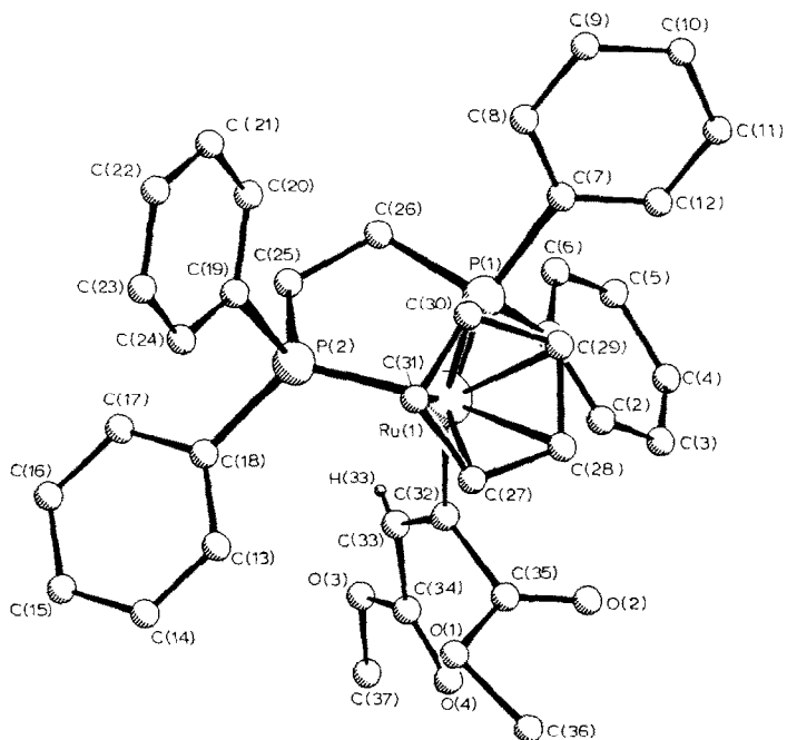
Fig. 1. A molecule of \text{Ru}\{(E)\text{-C}(\text{CO}_2\text{Me})=\text{CH}(\text{CO}_2\text{Me})\}(\text{dppe})(\eta\text{-C}_5\text{H}_5) ( 11 ), showing atom numbering scheme.
