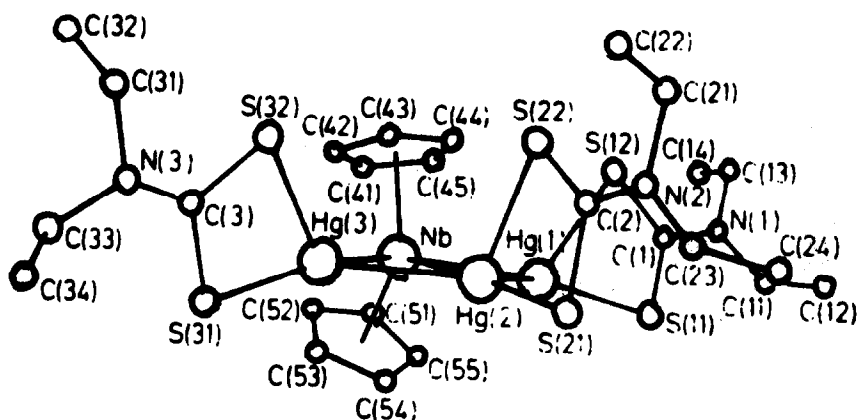
Figure 7. The Crystal Structure of [(\eta^5\text{-cp})_2\text{Nb}\{\text{HgS}_2\text{CN}(\text{C}_2\text{H}_5)_2\}_3] . Reproduced with permission from J. Chem. Soc. Dalton Trans. (Ref.31).
