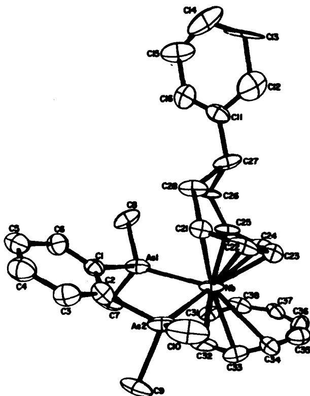
Figure 5. Molecular structure of [n^5\text{-cp}(\text{C}_8\text{H}_8)]\text{Nb}(n^4\text{-C}_8\text{H}_8)(\text{diars}) . Reproduced with permission from J. Am. Chem. Soc. (ref.28).
