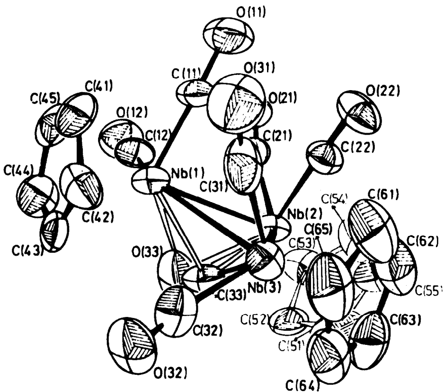
Figure. 11. Molecular structure of (\eta^5\text{-cp})_3\text{Nb}_3(\text{CO})_7 . Reproduced with permission from J. Am. Chem. Soc. (ref.56).
