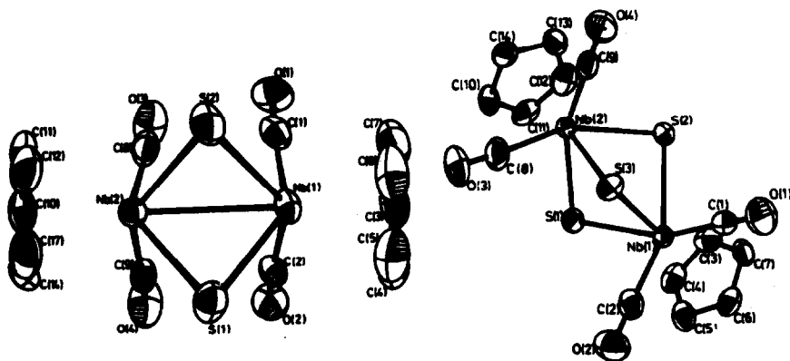
Figure. 10. Crystal structure of [(\eta^5\text{-cp})\text{Nb}(\text{CO})_2]_2(\mu\text{-S})_3 .
