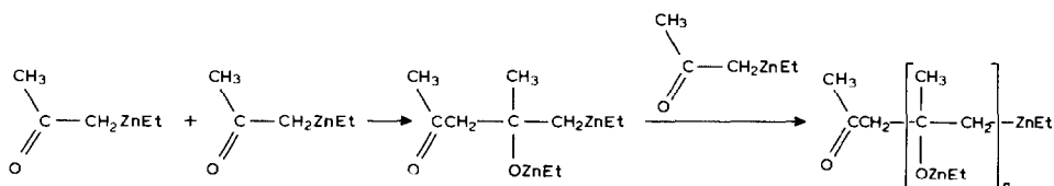
SCHEME 2. Proposed mechanism for the Grignard-like addition of a C-metallated zinc enolate over the \text{C}=\text{O} of another C-metallated zinc enolate.
