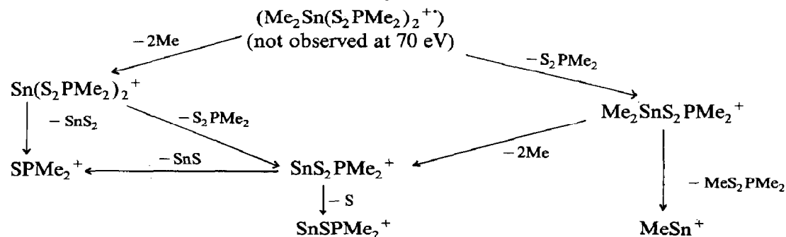
Scheme 1. Fragmentation pattern of Me 2 Sn(S 2 PMe 2 ) 2 + .
