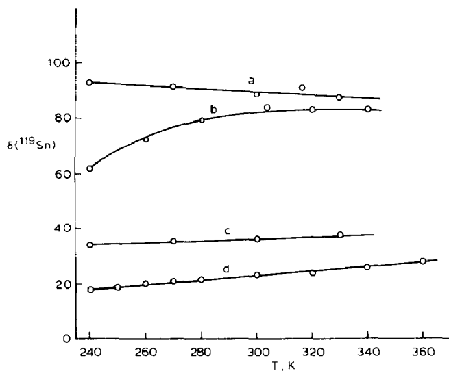
Fig. 1. Temperature dependence of \delta(^{119}\text{Sn}) of \text{Bu}_3\text{Sn}(\text{txin}) ((c) in \text{CDCl}_3 , (d) in pyridine) and of \text{Bu}_3\text{SnS}(1\text{-C}_{10}\text{H}_7) ((a) in \text{CDCl}_3 , (b) in pyridine).
