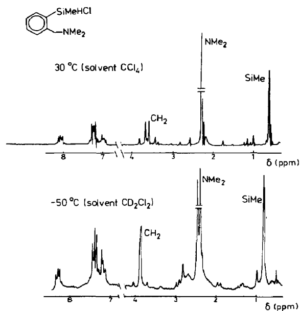
Fig. 2. The ^1\text{H} NMR spectra of \text{A}_{14} .
