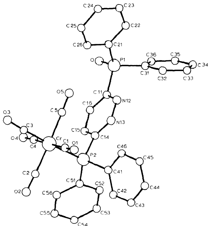
Fig. 1. Structure of \text{Cr}(\text{CO})_5\text{dppzO} .
