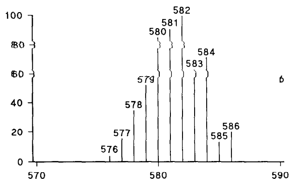
Fig. 3. Measured (a) and calculated (b) isotopic distribution for the [M + HgMe] ion.
