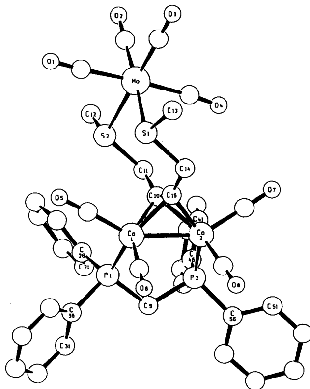
Fig. 1. The molecular structure of 1a showing the atom labelling system.
