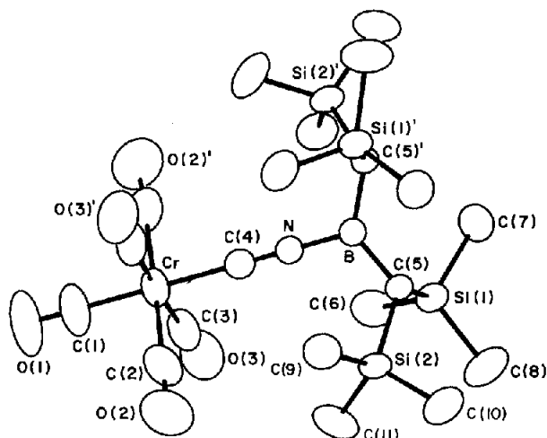
Fig. 1. The molecular structure of [\text{Cr}(\text{CO})_5(\text{CNBR}_2)] [ R = \text{CH}(\text{SiMe}_3)_2 ] ( 2a ).
