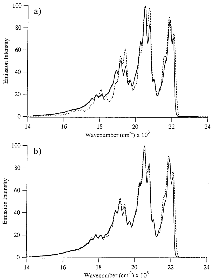
Fig. 11. The 15 K emission spectrum of hexafluoroacetylacetonatodimethylgold(III) (solid lines). The top panel show the 'best fit' with uncoupled normal modes (dotted lines.) The bottom panel shows the best fit with quadratically coupled normal modes ( \Gamma = 74 \text{ cm}^{-1} , 258 \text{ cm}^{-1} with \Delta_x = 1.44 , 1354 \text{ cm}^{-1} with \Delta_y = 1.52 and a coupling between the modes of k_{xy} = 116.5 \text{ cm}^{-1} ).
