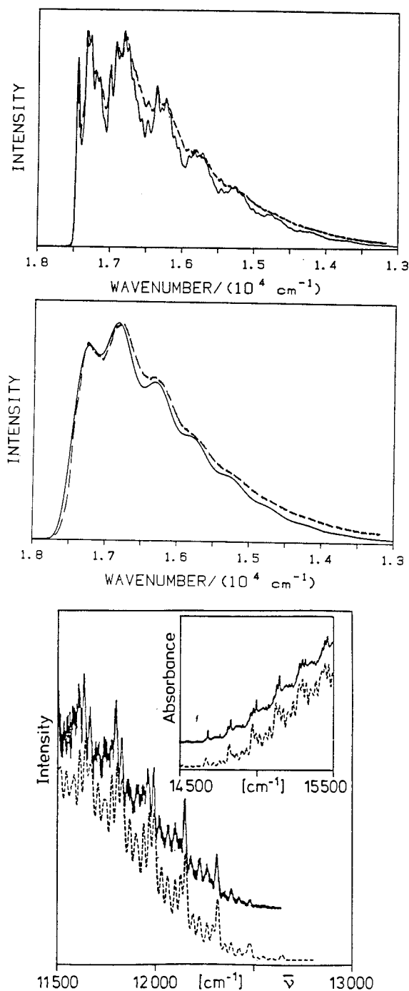
Fig. 9. Top and middle: the emission spectra (dotted lines) of \text{trans-W(N}_2)_2(\text{dppe})_2 (dppe = 1,2 bis(diphenylphosphino)ethane). The spectrum taken at 80 K, shown in the middle panel, appears to contain a single progression with a spacing of 500 \text{ cm}^{-1} . Lowering the temperature to 10 K resolves new features (top panel). The calculated low temperature spectrum ( \Gamma = 17.5 \text{ cm}^{-1} ) is given by the solid line in the middle panel. The emission spectrum of the 80 K sample is calculated using exactly the same parameters of frequencies and distortions but with a \Gamma of 80 \text{ cm}^{-1} (middle panel.) Bottom: the emission spectrum of ((\text{C}_2\text{H}_5)_2\text{N})_2[\text{Pd}(\text{MNT})_2] (mnt = \text{S}_2\text{C}_2(\text{CN})_2^{2-} ). The regular 26 \text{ cm}^{-1} spacing between the vibronic features is the beat frequency between the two most highly distorted modes in the molecule ( 162 \text{ cm}^{-1} and 188 \text{ cm}^{-1} ).
