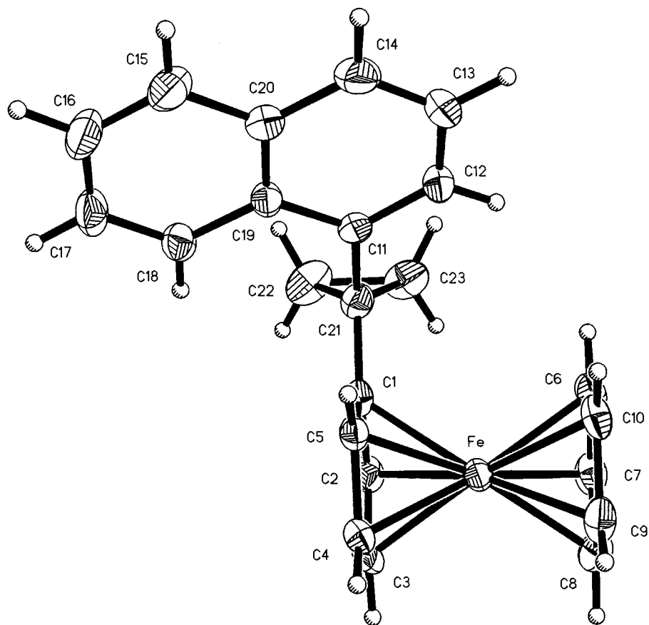
Fig. 3. Crystal structure of 9 . Selected bond lengths (Å): C 21 –C 22 = 1.517(6); C 21 –C 23 = 1.513(6); C 22 –C 23 = 1.492(8); and selected bond angles (°): C 22 –C 21 –C 23 = 59.0(3); C 21 –C 22 –C 23 = 60.4(3); C 22 –C 23 –C 21 = 60.6(3).
