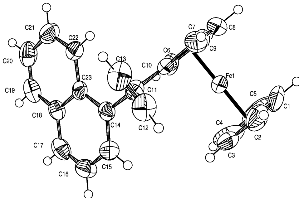
Fig. 1. Crystal structure of 6 . Selected bond lengths (Å): C 11 –C 12 = 1.498(5); C 11 –C 13 = 1.509(5); C 12 –C 13 = 1.272(6); and selected bond angles (°): C 12 –C 11 –C 13 = 50.0(2); C 13 –C 12 –C 11 = 65.4(3); C 12 –C 13 –C 11 = 64.5(3).
