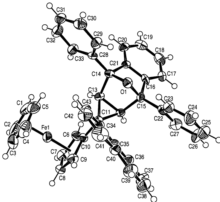
Fig. 4. Crystal structure of 11 . Selected bond lengths (Å): C_{11}-C_{12} = 1.519(6) ; C_{11}-C_{13} = 1.532(6) ; C_{12}-C_{13} = 1.513(6) ; and selected bond angles ( ^{\circ} ): C_{12}-C_{11}-C_{13} = 59.5(3) ; C_{13}-C_{12}-C_{11} = 60.7(3) ; C_{12}-C_{13}-C_{11} = 59.8(3) ; C_{34}-C_{11}-C_{10} = 113.9(4) ; C_{34}-C_{11}-C_{12} = 121.7(4) ; C_{34}-C_{11}-C_{13} = 125.7(4) .
