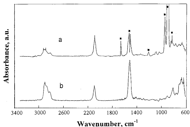
Fig. 4. FTIR spectrum of gaseous silicon-containing products resulting from LPD of SCB- d_2 obtained by (a) subtracting contributions of ethene, propene and SCB- d_2 (peaks designated ■ relate to a fraction of \text{SF}_6 ), and by (b) adding contributions of all the silicon-containing products as separated (Table 1) by the GC-FTIR technique. Irradiation conditions: SCB- d_2 (4 Torr), \text{SF}_6 (4 Torr), \text{N}_2 (38 Torr), fluence = 0.5 \text{J cm}^{-2} , 30% decomposition.
