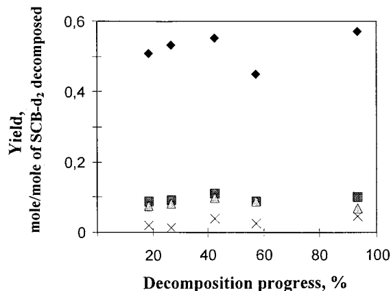
Fig. 3. Product distribution (in mol mol -1 of SCB-d 2 decomposed) in LPD of SCB-d 2 . Product designation: ◆ ethene, ■ propene, △ methylsilane (mostly D 2 HC–SiD 2 H), X dimethylsilane (SiC 2 D 3 H 3 ). 19% decomposition—SCB-d 2 (4.6 Torr), SF 6 (3 Torr), N 2 (55 Torr), 2000 pulses; 27% decomposition—SCB-d 2 (3.3 Torr), SF 6 (3 Torr), N 2 (55 Torr), 5000 pulses; 43% decomposition—SCB-d 2 (4.1 Torr), SF 6 (6.0 Torr), N 2 (38 Torr), 60 pulses; 57% decomposition—SCB-d 2 (4.0 Torr), SF 6 (4.0 Torr), N 2 (38 Torr), 1500 pulses; 94% decomposition—SCB-d 2 (3.0 Torr), SF 6 (3.0 Torr), N 2 (38 Torr), 2000 pulses; all runs with fluence of 0.5 J cm -2 .
