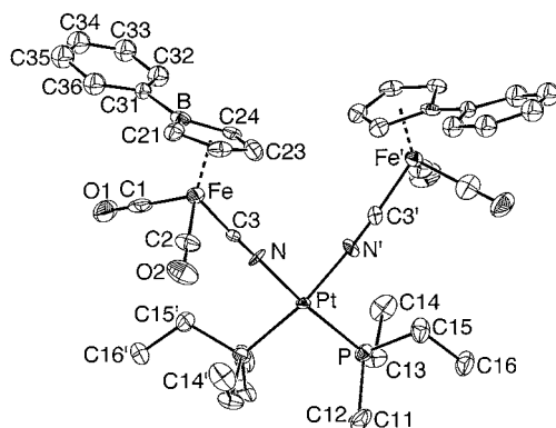
Fig. 1. PLATON-plot [16] of cis - \{[\text{Fe}](\mu\text{-CN})\}_2\text{Pt}(\text{PEt}_3)_2 ( 2 ). Displacement ellipsoids are drawn at 30% probability.
