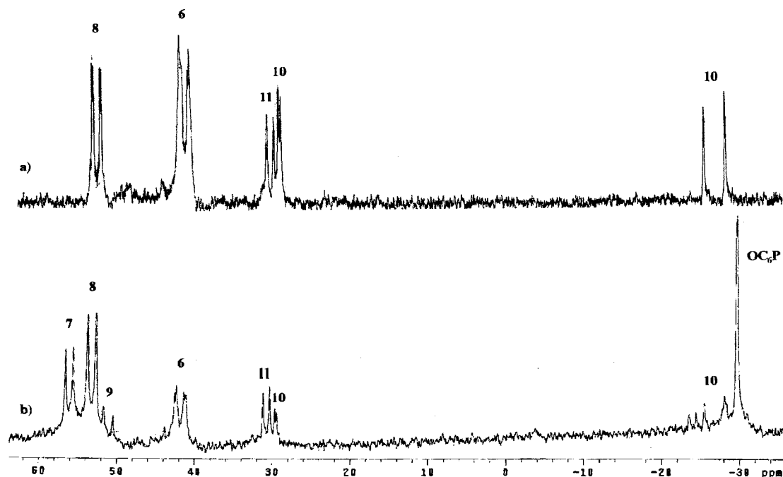
Fig. 2. ^{31}\text{P}\{^1\text{H}\} -HPNMR spectrum of reaction of [\text{Rh}(\text{acac})(\text{CO})_2]/\text{rac-OC}_6\text{P} with \text{CO} and \text{H}_2 : (a) \text{P-P/Rh} = 1 ; (b) \text{P-P/Rh} = 2 .
