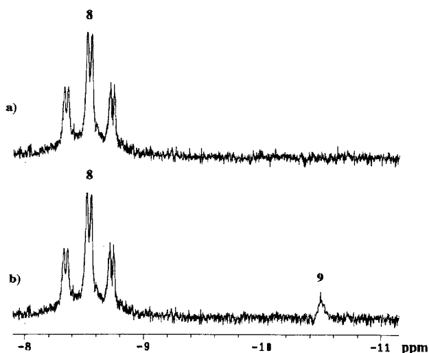
Fig. 4. ^1\text{H} -HPNMR spectrum of reaction of [\text{Rh}(\text{acac})(\text{CO})_2]/\text{rac-OC}_6\text{P} with CO and H 2 in the high-field region: (a) \text{P-P/Rh} = 1 ; (b) \text{P-P/Rh} = 2 .
