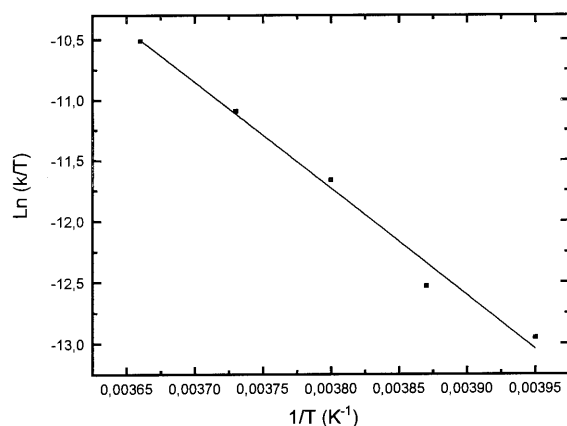
Fig. 3. Eyring plot for the tautomerisation process [(C 5 Me 5 )Ru(H 2 )(PEt 3 ) 2 ] + (7) → [(C 5 Me 5 )RuH 2 (PEt 3 ) 2 ] + (3b) in CD 2 Cl 2 .
