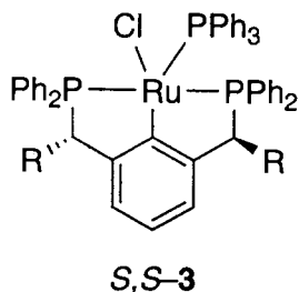
Scheme 1.
