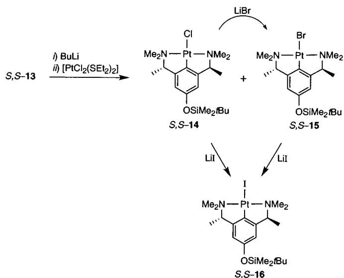
Scheme 7.
