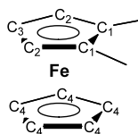
Scheme 1. Atom numbering scheme used for 1,2-disubstituted ferrocene compounds.
