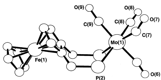
Fig. 2. Molecular structure (Pluton diagram) of 1,2- \text{Fc}''(\text{CH}_2\text{PH}_2)_2\text{-Mo}(\text{CO})_4 ( 8 ) with all hydrogen atoms omitted.
