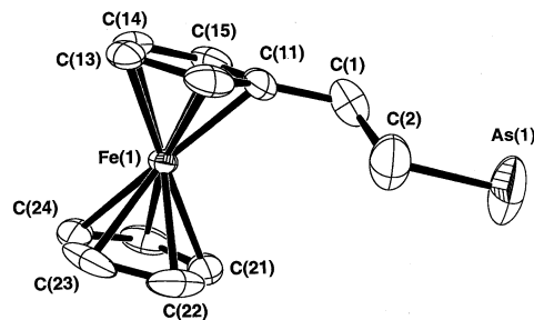
Fig. 1. Molecular structure of FcCH 2 CH 2 AsH 2 ( 7 ), showing the atom numbering scheme. Thermal ellipsoids are at the 50% probability level.
