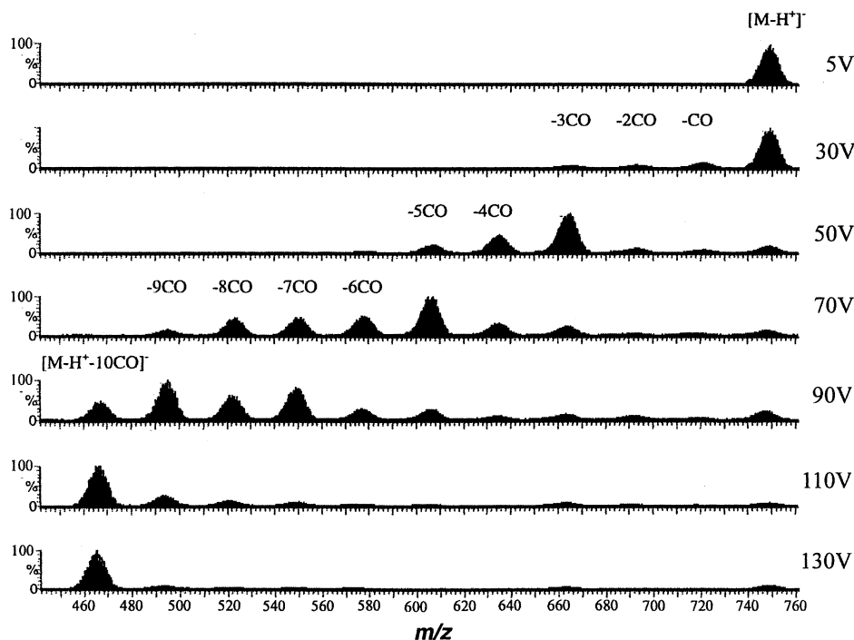
Fig. 3. Negative ion ES spectra (in methanol with added sodium methoxide) of 1,1'-Fc'[CH 2 PH 2 Mo(CO) 5 ] 2 ( 10 ) at various cone voltages, showing the loss of all ten CO ligands with increasing cone voltage.
