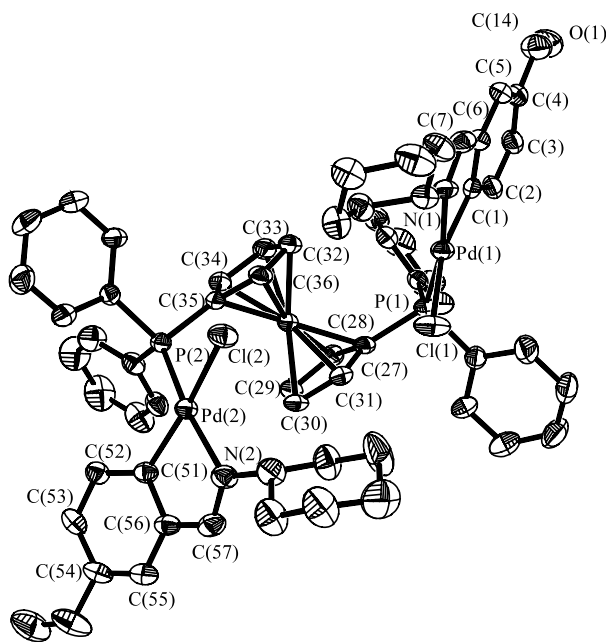
Fig. 3. Molecular structure of [\{\text{Pd}[5\text{-(COH)C}_6\text{H}_3\text{C(H)=NCy-C2,N}]\text{(Cl)}\}_2\{\mu\text{-(Ph}_2\text{PC}_5\text{H}_4\text{)}_2\text{Fe}\}] ( 6 ), with labelling scheme. Hydrogen atoms have been omitted for clarity.
