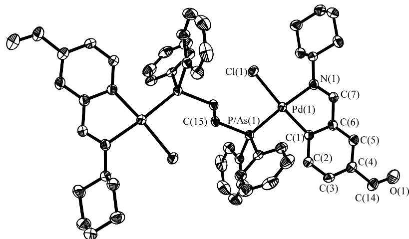
Fig. 4. Molecular structure of [\{\text{Pd}\{5\text{-(COH)C}_6\text{H}_3\text{C(H)=NCy-C2,N}\}(\text{Cl})\}_2(\mu\text{-Ph}_2\text{PCH}_2\text{CH}_2\text{AsPh}_2)] ( 9 ), with labelling scheme. Hydrogen atoms have been omitted for clarity.
