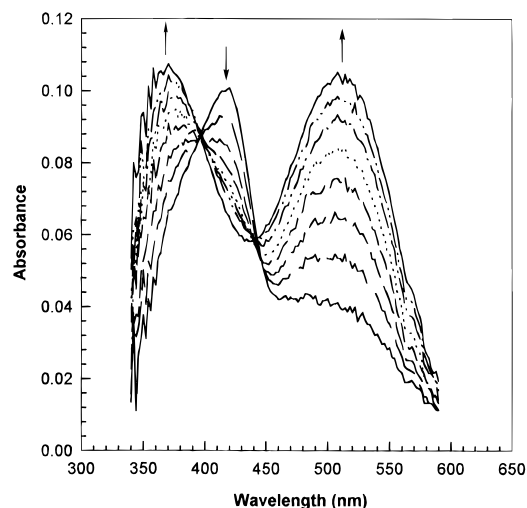
Figure 1. Typical kinetic UV–vis spectra for the ring-closure reaction of W(CO)_5bpy in supercritical CO_2 with 7% methanol recorded at 70 °C, 13.5 MPa, and \Delta t = 15 s.
