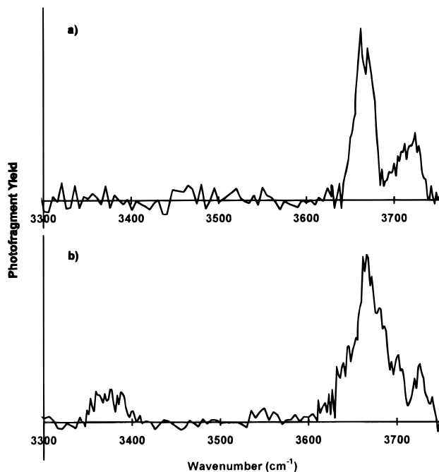
Figure 5. Vibrational predissociation spectra of HDNO_3^+ formed (a) in a glow discharge and (b) by electron beam ionization of the free jet expansion.
