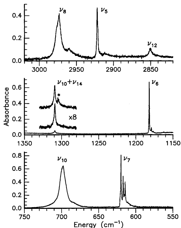
Figure 2. Most intense vibrational transitions of the DMZ/Ar sample having a dilution ratio of 1/1000 recorded with an instrument resolution of 0.25 \text{ cm}^{-1} at 12 K. Assignments of the vibrational transitions were made from the gas-phase data of Coats et al. In the middle panel, the \nu_{10} + \nu_{14} band is shown in an exaggerated fashion. The uppermost exaggerated spectra display an additional peak, indicated by the asterisk, due to contamination by methane.
