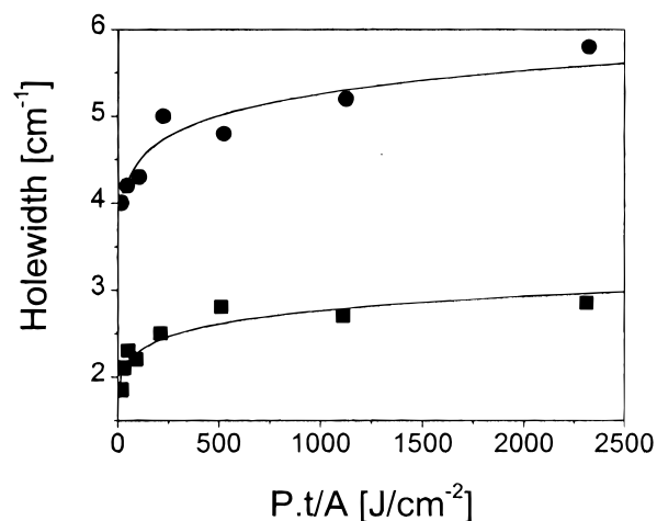
Figure 2. Hole widths measured in absorption of Chl. tepidum as a function of the burning fluence density \delta_{\text{HB}} = \delta_{\text{HB}}(Pt/A) , where P = burning power, t = burning time, and A = area, at anaerobic (squares) and aerobic (circles) conditions at 4.2 K at 780 nm.
