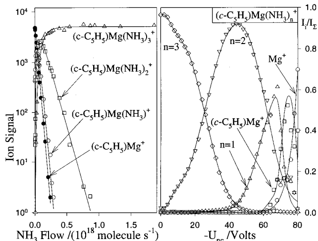
Figure 4. (Left) Experimental data recorded for the reaction of (c\text{-C}_5\text{H}_5)\text{Mg}^+ with ammonia in helium buffer gas at 294 \pm 3 K and 0.35 \pm 0.01 Torr. The (c\text{-C}_5\text{H}_5)\text{Mg}^+ ions were produced in a low-pressure ion source by electron impact dissociative ionization of magnesocene vapor at 50 eV. The solid lines represent a fit to the experimental data with the solution to the differential equations appropriate for the sequential addition reactions. Rate coefficients derived from the fit are given in Table 1. (Right) Results of multicollision CID experiments. The flow of ammonia is 1.0 \times 10^{18} molecules \text{s}^{-1} .
