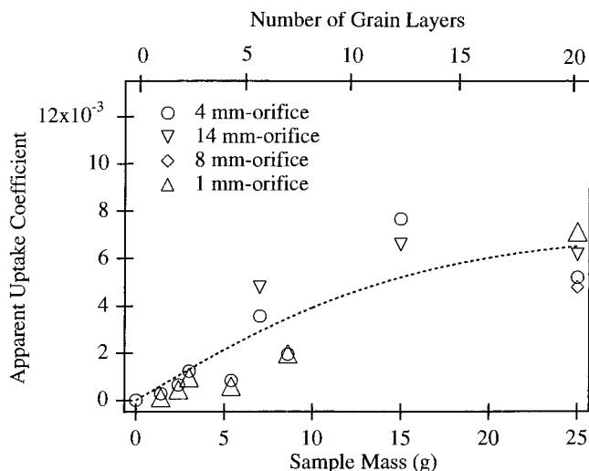
Figure 9. Results of monodisperse grain experiments (grain size 0.35 mm) using different orifice sizes. The dashed line is a fit obtained using the diffusion model proposed by Keyser and co-workers 13 using the value for the true uptake coefficient of 1.3 \times 10^{-4} .
