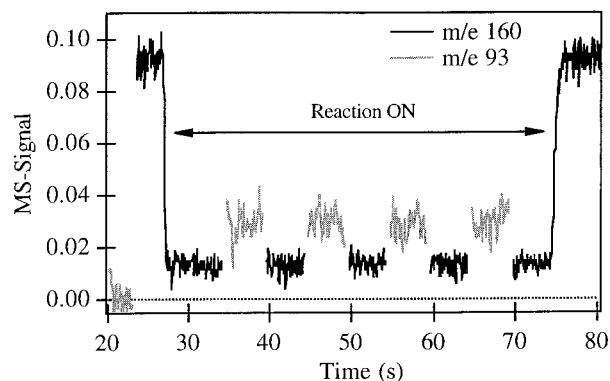
Figure 2. Steady-state experiment on the reaction of Br 2 + KNO 2 (reaction 6) performed using the 14 mm orifice with a Br 2 flow of 3.8 × 10 14 molecules s -1 . During this experiment we monitored the MS signal at m/e 93 (BrN + ) and at m/e 160 (Br 2 + ).
