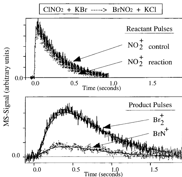
Figure 8. Pulsed-valve experiment of \text{ClNO}_2 on \text{KBr} (5 g of powder) performed using the 14 mm orifice. From this experiment we are able to measure the uptake coefficient by directly fitting the reactive \text{ClNO}_2 pulse to an exponential decay ( \gamma = 0.01 ). The \text{Br}_2 yield per loss of \text{ClNO}_2 is determined to be 0.61 by comparing the integrals of the reactant and product signals. \text{BrNO}_2 is detected at mass m/e 93. The solid lines are fits obtained using a two-parameter model (see text).
