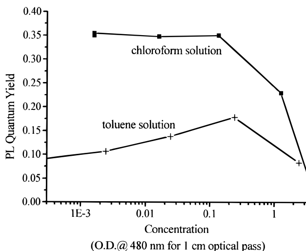
Figure 7. Fluorescence quantum yields, QE, of DOO-PPV in chloroform and toluene solutions with various concentrations at room temperature. At low concentration, the QE in toluene solution decreases as dilution, but that in chloroform solution remains the same.
