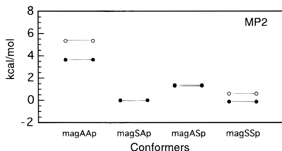
Figure 8. Total free energy differences in chloroform for the protonated N,N' -methylacetyl-guanidine conformers considered with respect to magSAp (see Scheme 1) obtained at the MP2 (black circles) level with the 6-311++G** basis set. The potential energy differences in vacuo (empty circles) are also displayed. Same remarks as in Figure 1.
