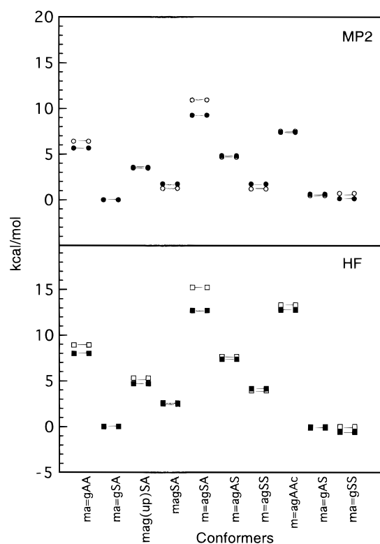
Figure 6. Total free energy differences in chloroform for the neutral N,N' -methylacetyl-guanidine conformers considered with respect to ma=gSA obtained at the HF (black squares) and MP2 (black circles) levels with the 6-311++G** basis set. The potential energy differences in vacuo at both levels (empty markers) are also displayed. Same remarks as in Figure 1.
