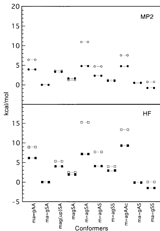
Figure 5. Total free energy differences in water for the neutral N,N' -methylacetyl-guanidine conformers considered with respect to ma=gSA (see text and Scheme 3) obtained at the HF (black squares) and MP2 (black circles) levels with the 6-311++G** basis set. The potential energy differences in vacuo at both levels (empty markers) are also displayed. Same remarks as in Figure 1.
